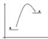
endotherm
