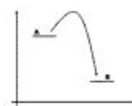
exotherm
